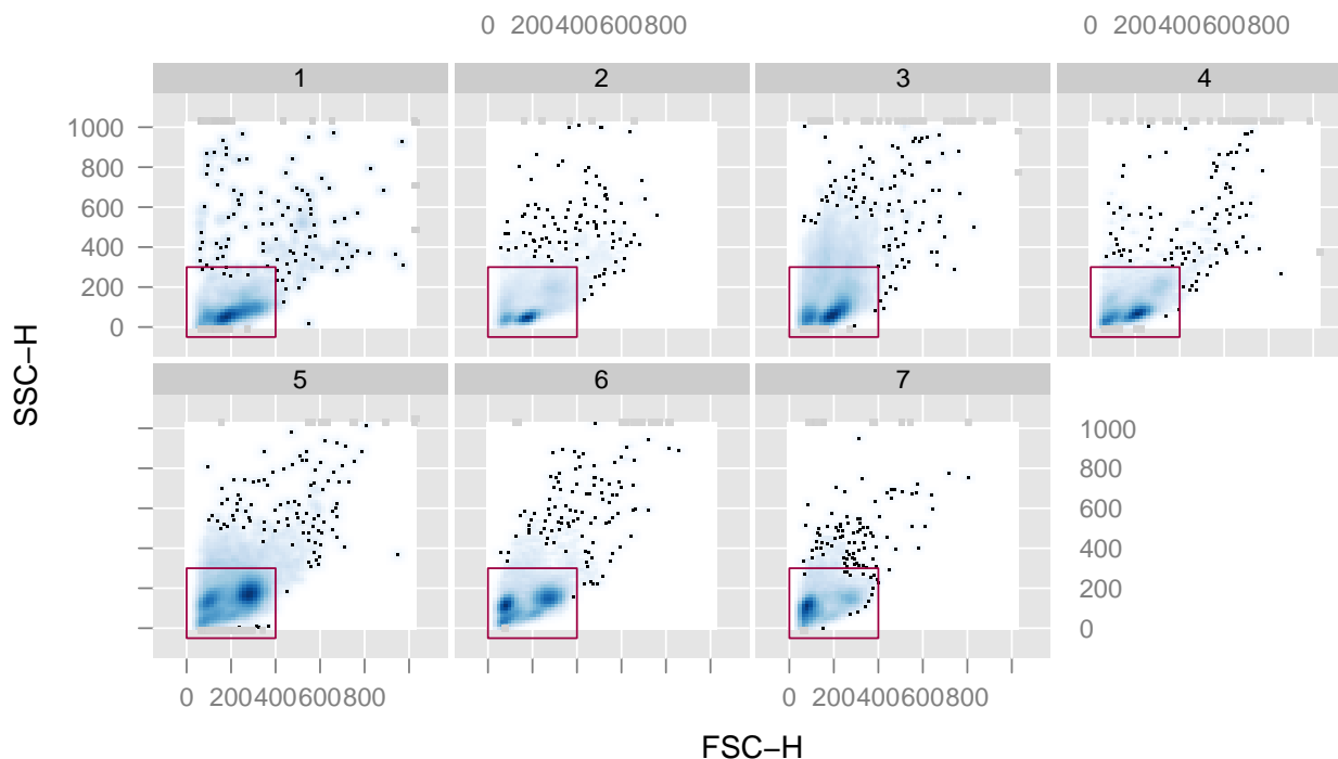
Figure 1: A simple rectangleGate visualization in the FSC-H-SSC-H xyplo.
