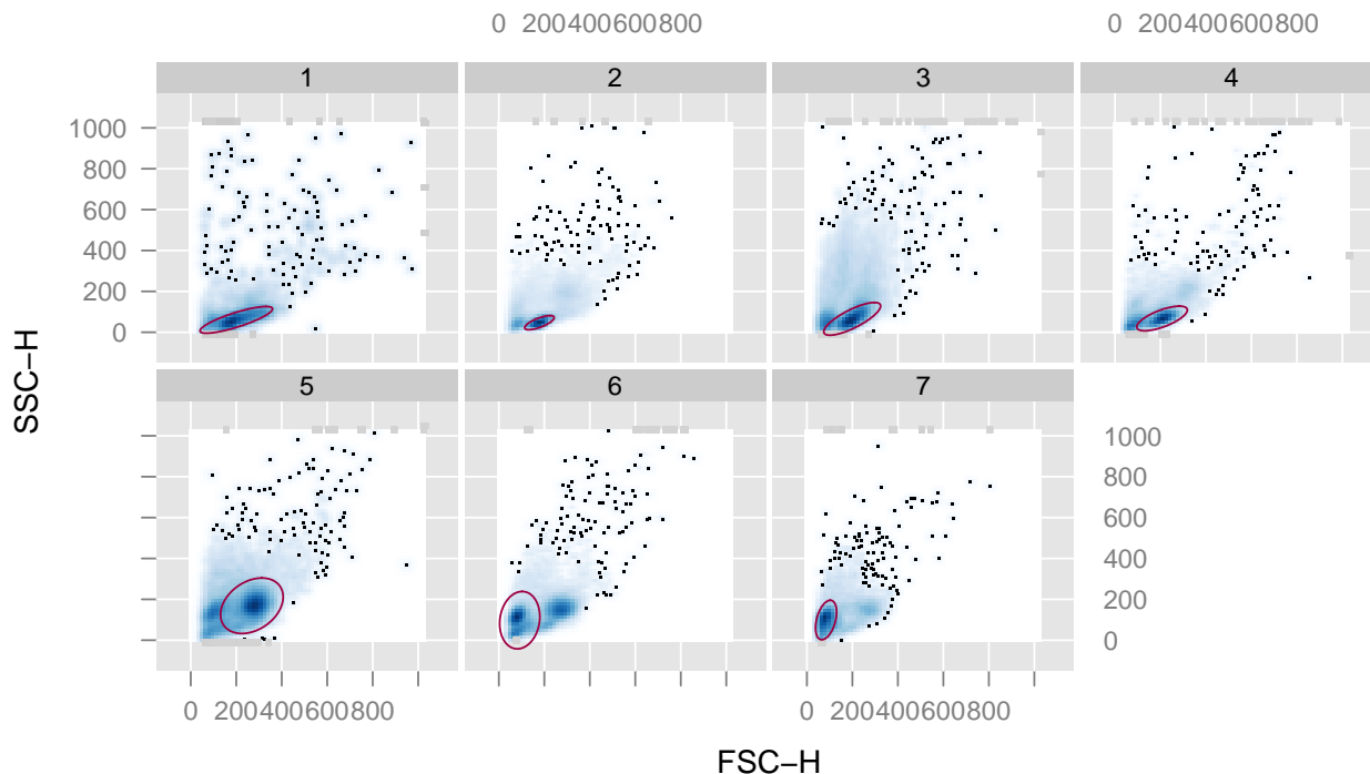
Figure 5: Gate defined by norm2Filter in the FSC-H and FL4-H channels.
