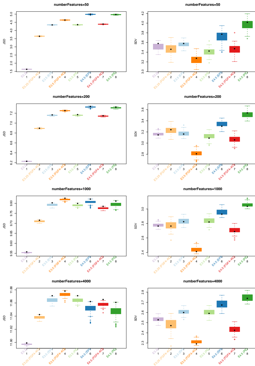
Figure 35: Jensen-Shannon divergences
