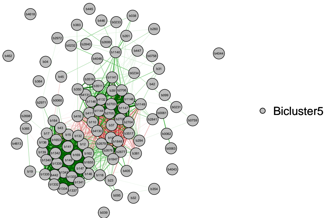
Figure 8: Network for the fifth bicluster identified in the Escherichia coli data.
