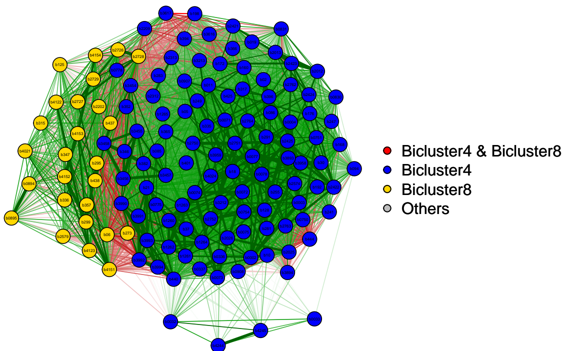
Figure 9: Network for the fourth and eighth biclusters identified in the Escherichia coli data.
