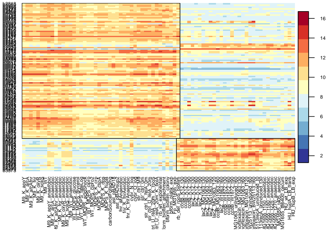
Figure 7: Heatmap for the fourth and eighth biclusters identified in the Escherichia coli data. Bicluster #4 (topeft) consists of 108 genes and 44 conditions, and bicluster #8 (bottom right) consists of 26 genes and 33 conditions
